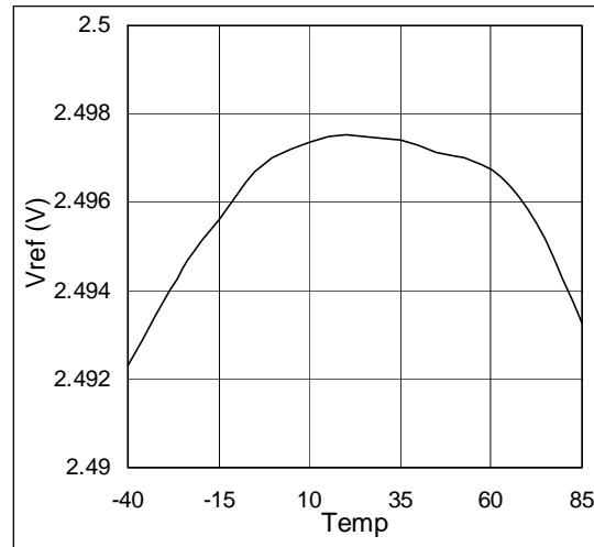
Figure 9. V_{REF} vs. Temperature; V_{DD} = 3.6V , AMODE = 1 , SGL/DIFF = 1 .
