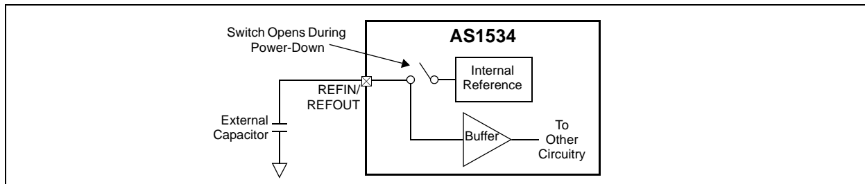
Figure 22. Internal Reference During Power-Down
