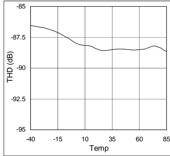
Figure 7. THD vs. Temperature; V_{DD} = 3.6V , AMODE = 1 , SGL/DIFF = 1 .
