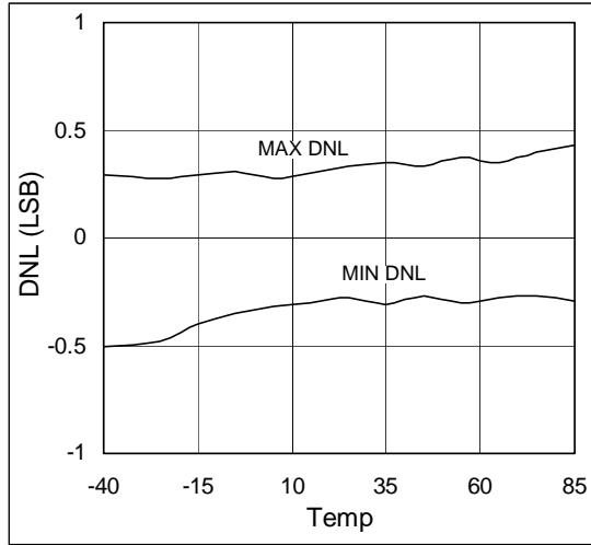
Figure 6. DNL vs. Temperature; V_{DD} = 3.6V , AMODE = 1 , SGL/DIFF = 1 .
