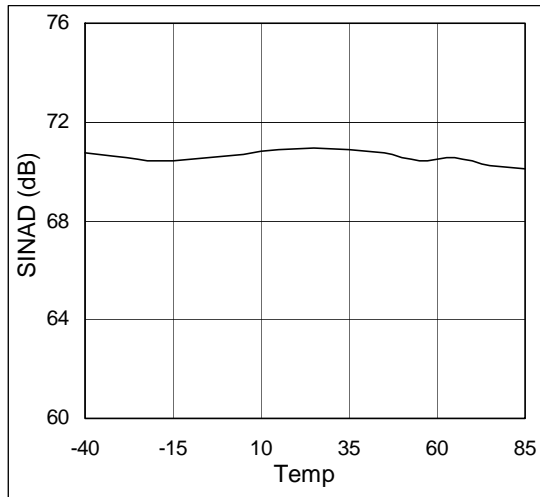
Figure 8. SINAD vs. Temperature; V_{DD} = 3.6V , AMODE = 1 , SGL/DIFF = 1 .
