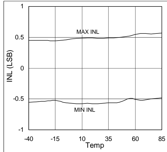
Figure 5. INL vs. Temperature; V_{DD} = 3.6\text{V} , AMODE = 1 , SGL/DIFF = 1 .
