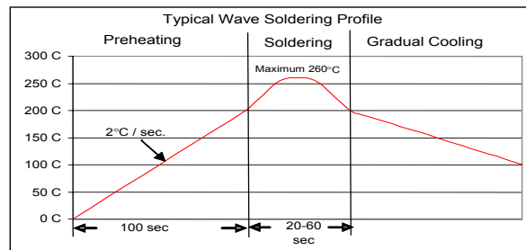
TYPICAL WAVE SOLDERING PROFILE
