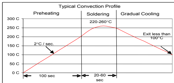
TYPICAL CONVECTION PROFILE
