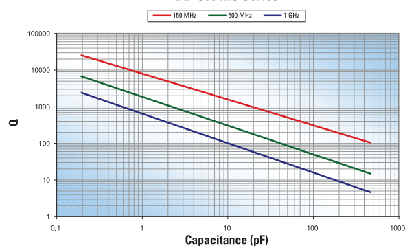
Q vs Capacitance DLI C08 MS Series
