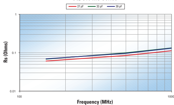
ESR vs Frequency DLI C10 MS Series
