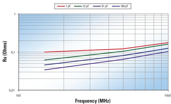
ESR vs Frequency DLI C11 MS Series
