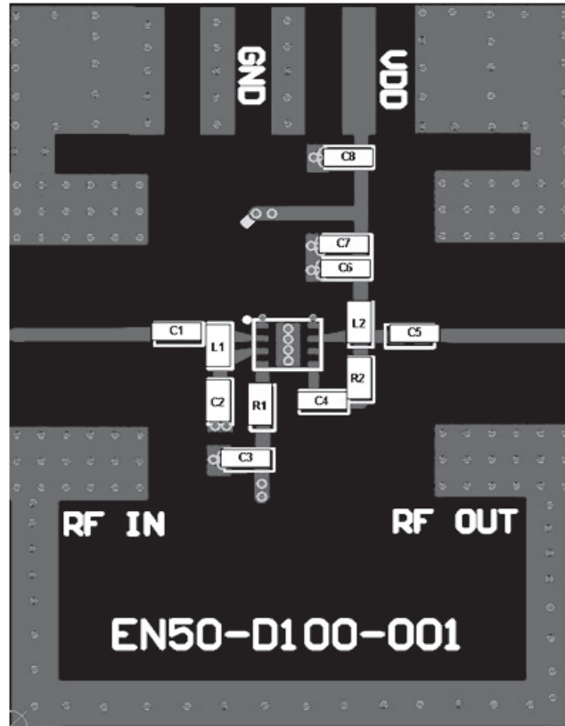
Figure 15. SKY67100-396LF Evaluation Board Assembly Diagram
