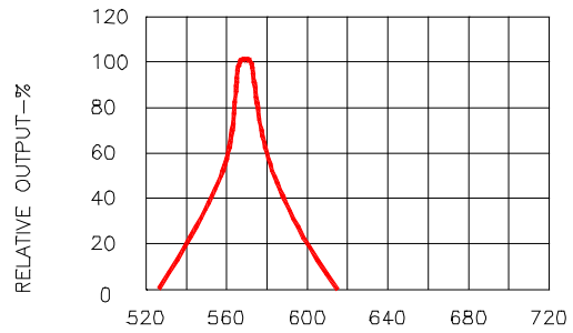
Fig.2 SPECTRAL RESPONSE
