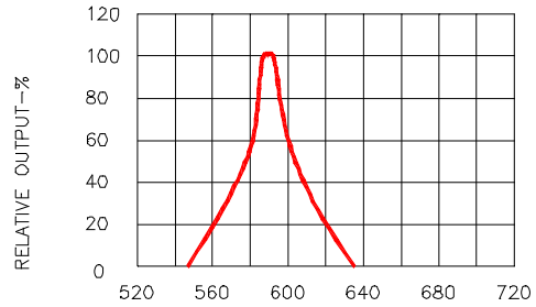
WAVELENGTH(λ)—nm
