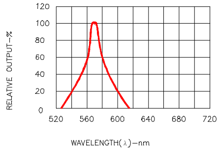
Fig.2 SPECTRAL RESPONSE
