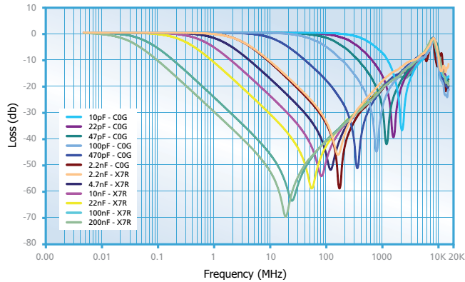
E01 & E07 Insertion Loss
