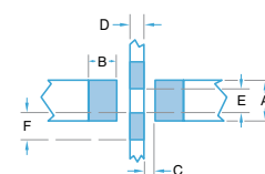
Recommended solder lands
