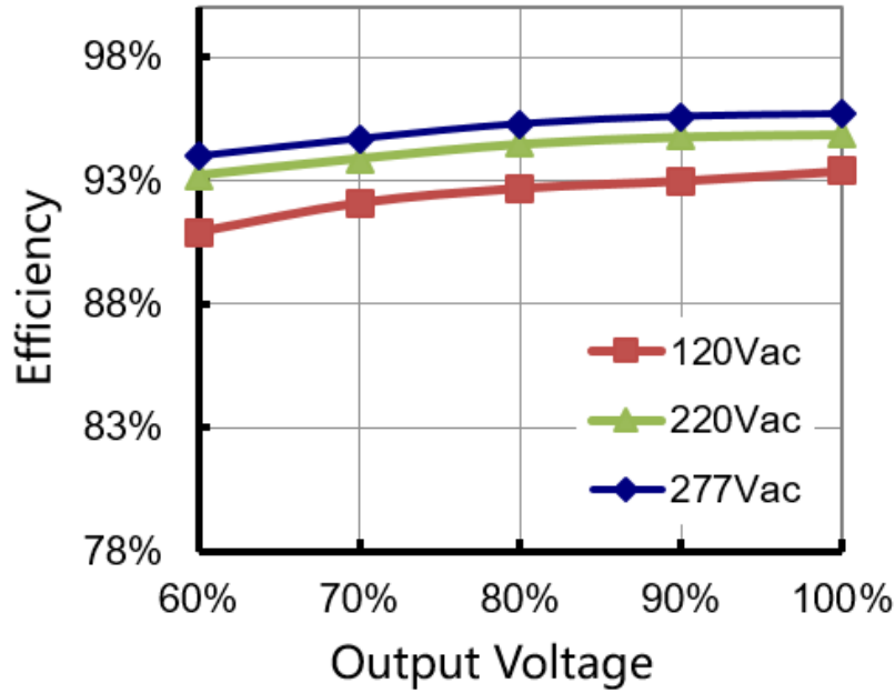
Efficiency vs. Output Voltage
