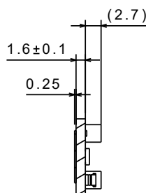
Section view A-A Scale:2:1
