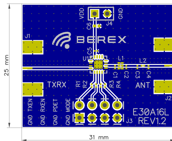
Figure 4: 8TR8218 Reference Design Schematic and PCB Layout
