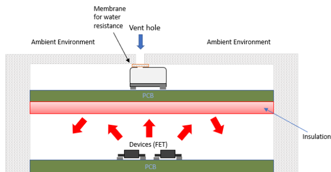
Figure 4. Thermal Isolation
