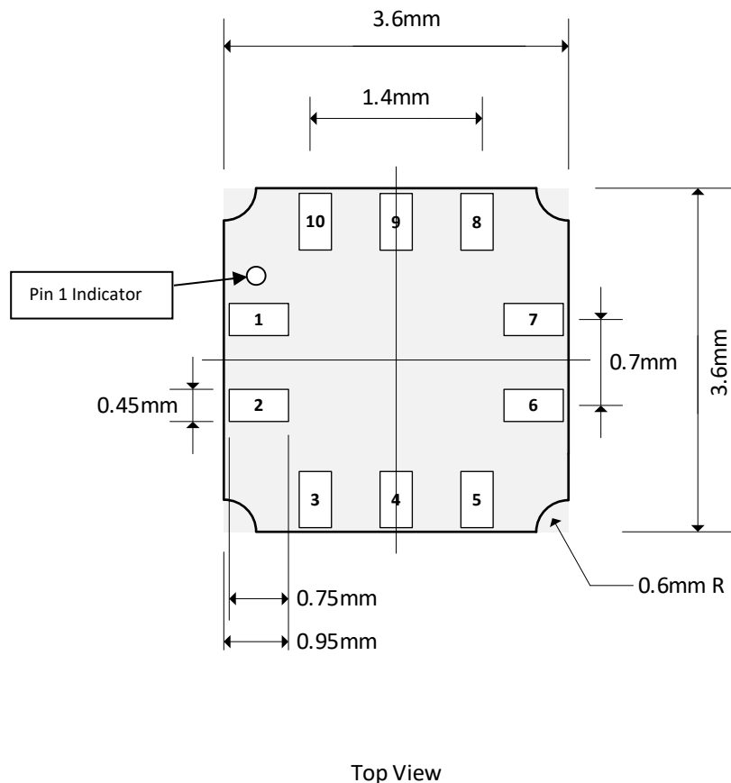
Figure 13. ICP-10125 recommended PCB land pattern
