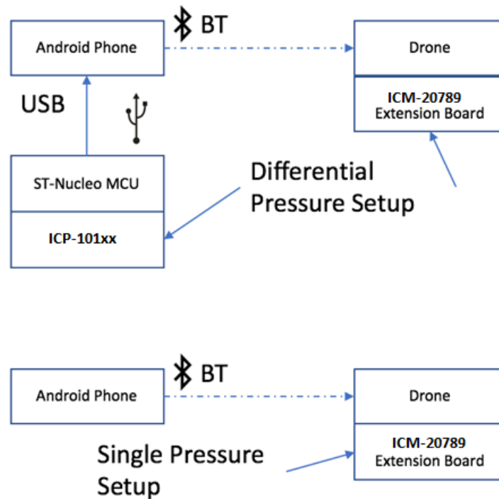
Figure 5. Experiment setup
