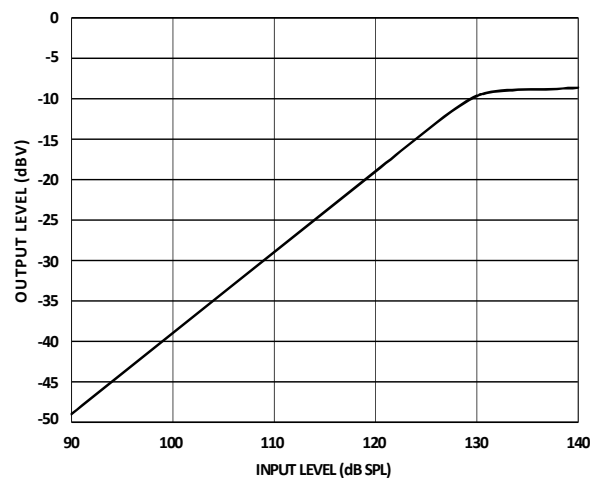
Figure 6. Linearity
