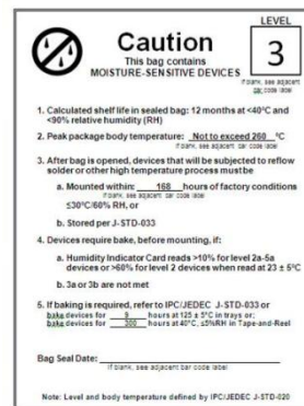
Moisture-Sensitivity Caution Label
