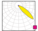
TF Narrow forward throw beam optimized for European tunnels
