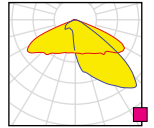
MEW Extremely low glare fulfilling EN13201 M-class requirements for wet road surfaces in North Europe
