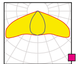
CAT-B Narrow catenary street light beam optimized for EN13201 M-classes and tilted poles
