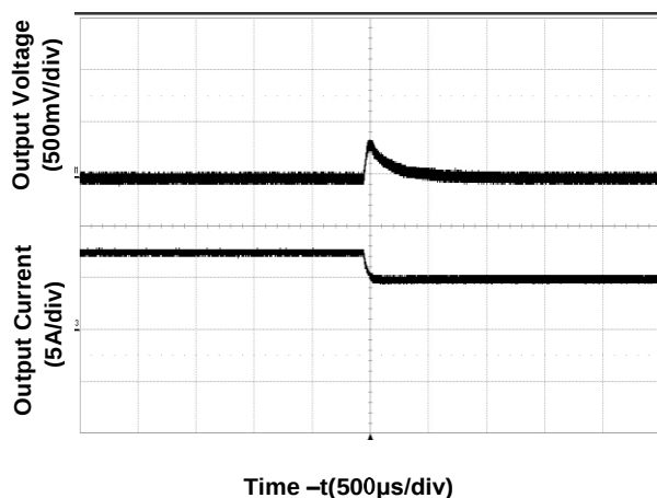
Figure 7. Transient Load Response (Typical Vin, load current steps from 75% to 50% at a slew rate 0.1A/μs)
