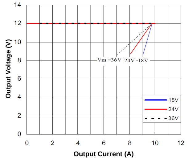
Figure 10. Output Characteristics
