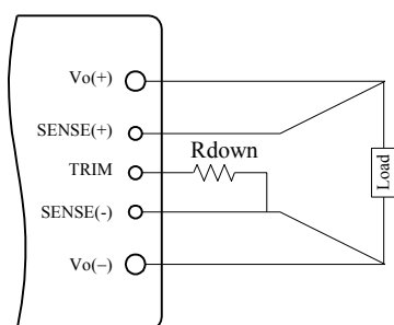
Figure 17. Circuit to Decrease Output Voltage
