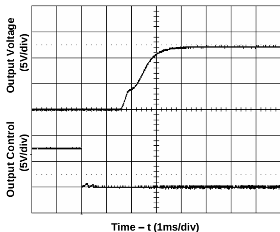
Figure 3. Start-Up from Enable Control (Typical Input voltage and full load)
