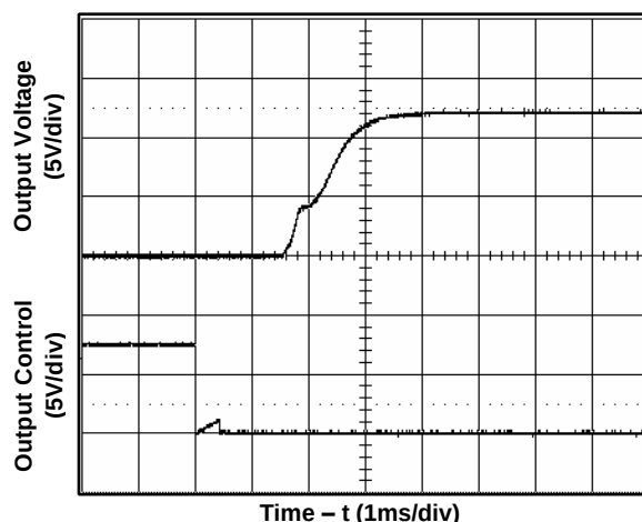
Figure 4. Start-Up from Enable Control (Typical Input voltage and zero load)
