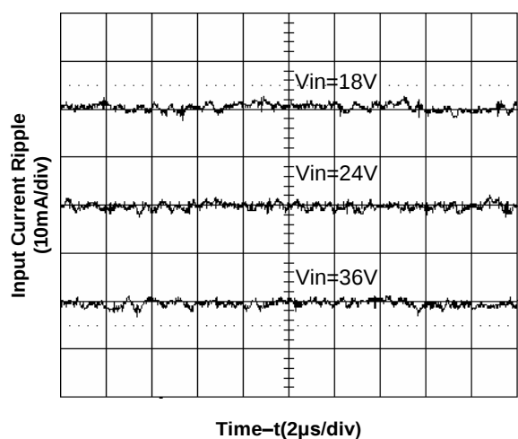
Figure 6. Input Reflected Ripple at Full Load
