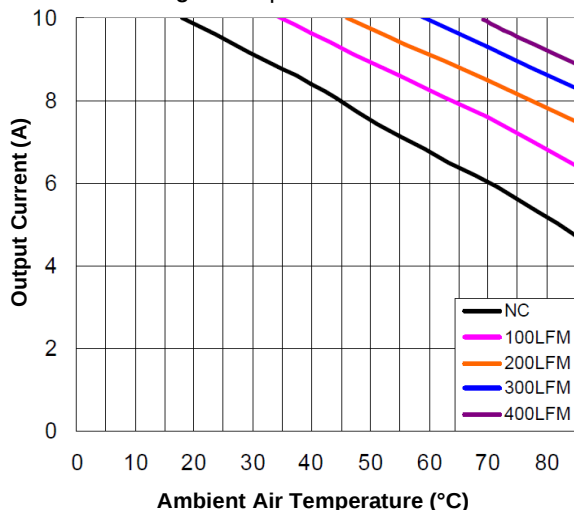
Figure 11. Current Derating Curve for Airflow Direction 3 (Ref. Figure 12 for Airflow Direction; typical V_{in} , open frame, unit soldered onto a fixture board.)
