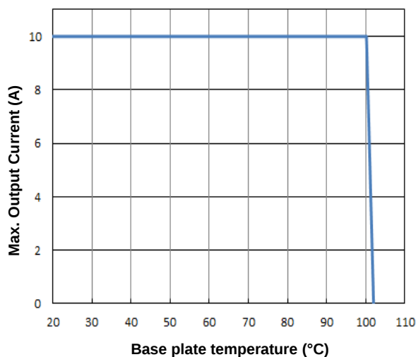
Figure 13. Current Derating Curve for Base plate (typical V_{in} with Base plate; solder interface)
