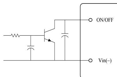
Figure 15. Open Collector Enable Circuit
