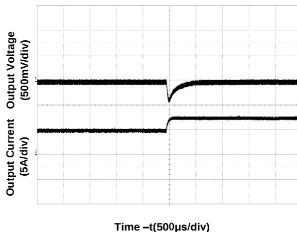
Figure 8. Transient Load Response (Typical Vin, load current steps from 50% to 75% at a slew rate 0.1A/μs)
