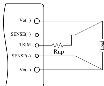
Figure 18. Circuit to Increase Output Voltage
