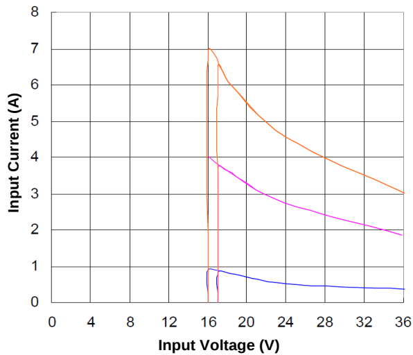
Figure 9. Input Characteristics
