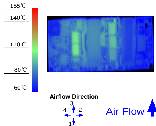
Figure 12. Thermal Image for Airflow Direction 3 (9.3 A output, 55°C ambient, 200LFM, typical V_{in} , open frame, unit soldered onto a fixture board.)
