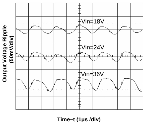
Figure 5. Output Ripple Voltage at Full Load
