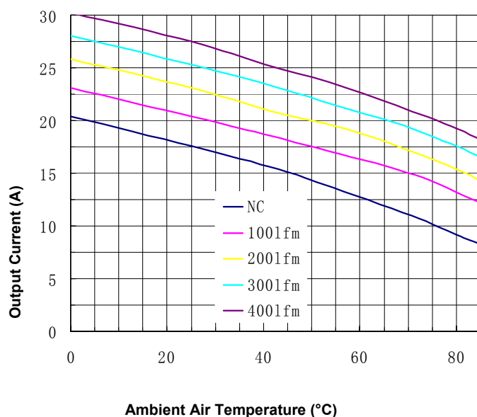
Figure 13. Current Derating Curve for Airflow Direction 2 (Ref. Fig.14 for Airflow Direction; Vin = 36V, open frame unit)
