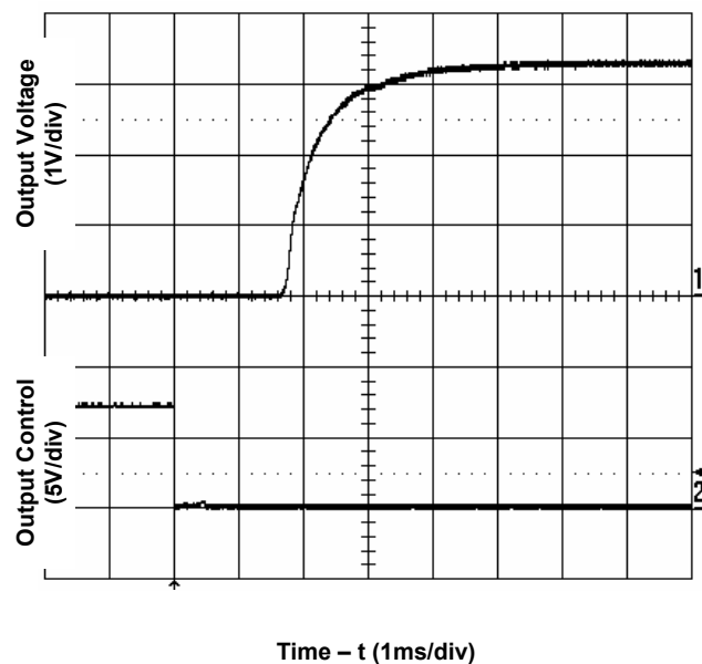
Figure 3. Start-Up from Enable Control
