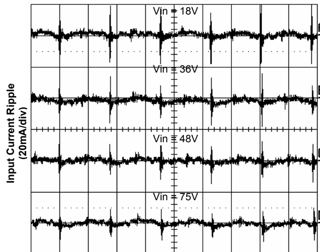
Time - t (2µs/div) Figure 6. Input Reflected Ripple Current at 30A Load
