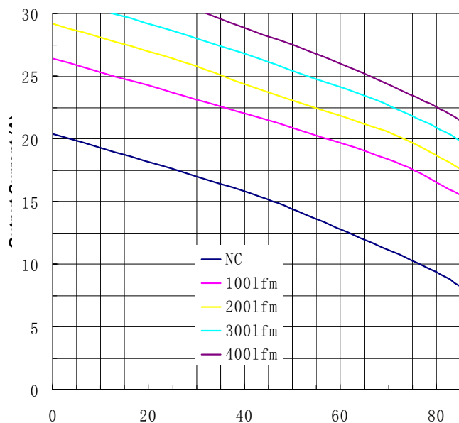
Figure 11. Current Derating Curve for Airflow Direction 3 (Ref. Fig. 12 for Airflow Direction; Vin = 36V, open frame unit)
