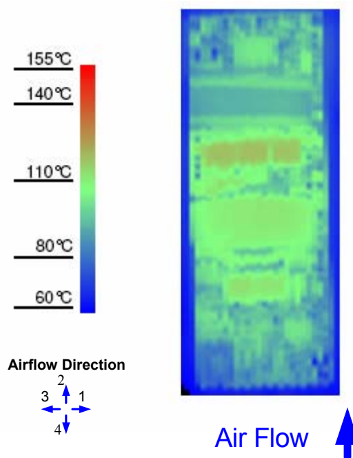
Figure 14. Thermal Image for Airflow Direction 2 (17.5A output, 55°C ambient, 200 LFM, Vin = 36V)
