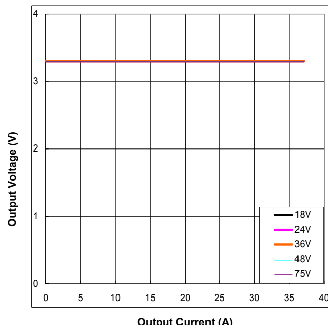
Figure 10. Output Characteristics
