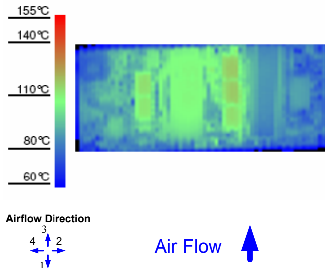
Figure 12. Thermal Image for Airflow Direction 3 (21.5A output, 55°C ambient, 200 LFM, Vin = 36V)
