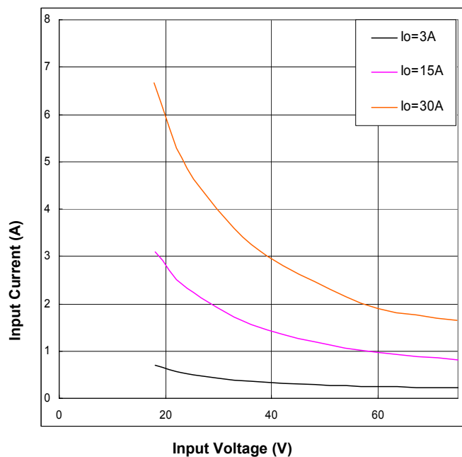
Figure 9. Input Characteristics
