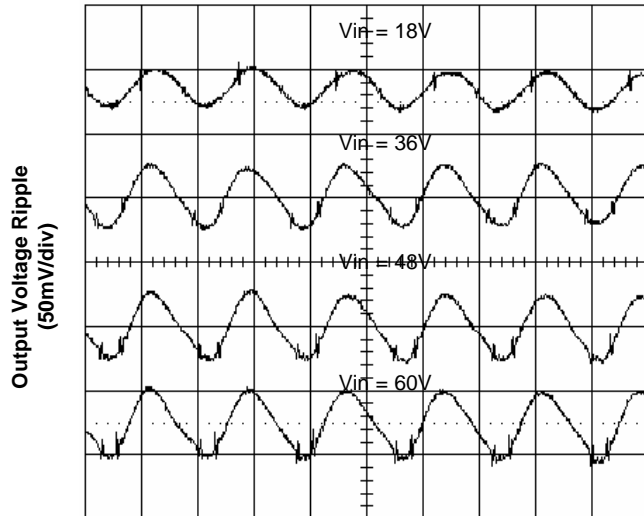
Figure 5. Output Ripple Voltage at 9A Load
