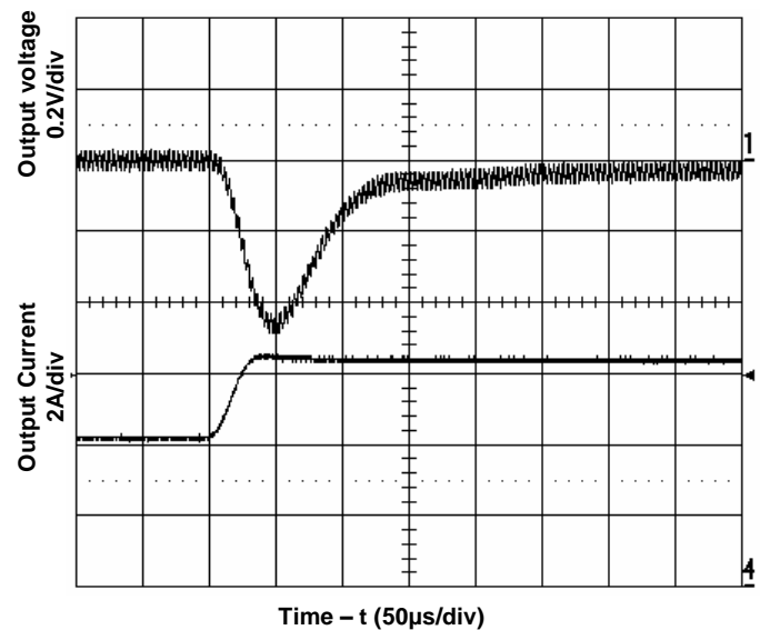
Figure 8. Transient Load Response
