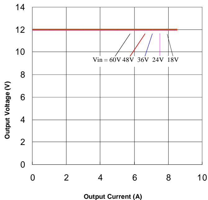
Figure 10. Output Characteristics
