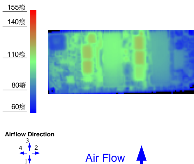
Figure 12. Thermal Image for Airflow Direction 3 (9A output, 55°C ambient, 200 LFM, V_{in} = 36V )
