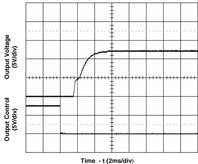
Figure 4. Start-Up from Enable Control
