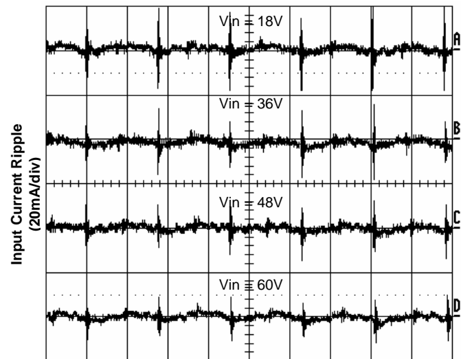
Figure 6. Input Reflected Ripple Current at 9A Load
