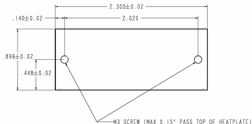
Figure 24. Converter with optional baseplate
