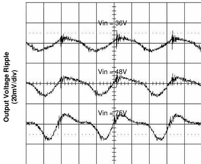
Figure 5. Output Ripple Voltage at 25A Load
