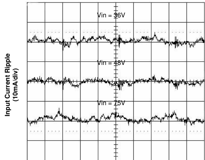
Figure 6. Input Reflected Ripple Current at 25A Load
