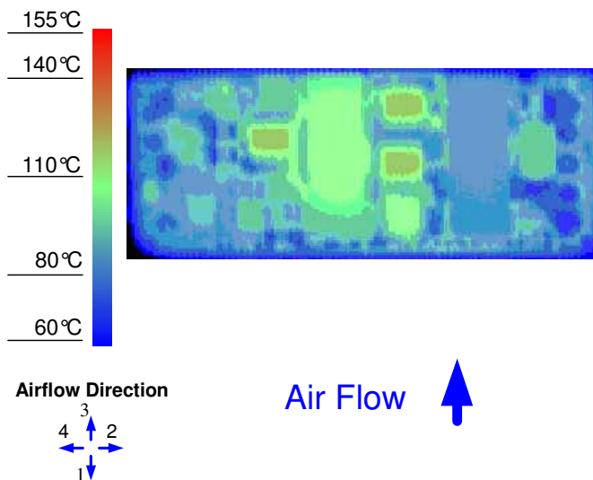
Figure 12. Thermal Image for Airflow Direction 3 (21A output, 55°C ambient, 200 LFM, Vin = 48V open frame unit using socket interface)
