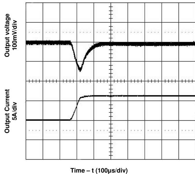
Figure 8. Transient Load Response
