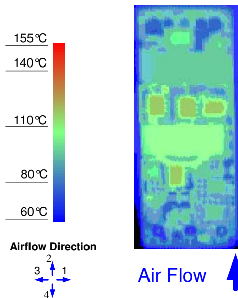
Figure 14. Thermal Image for Airflow Direction 2 (18.8A output, 55°C ambient, 200 LFM, Vin = 48V open frame unit using solder interface)
