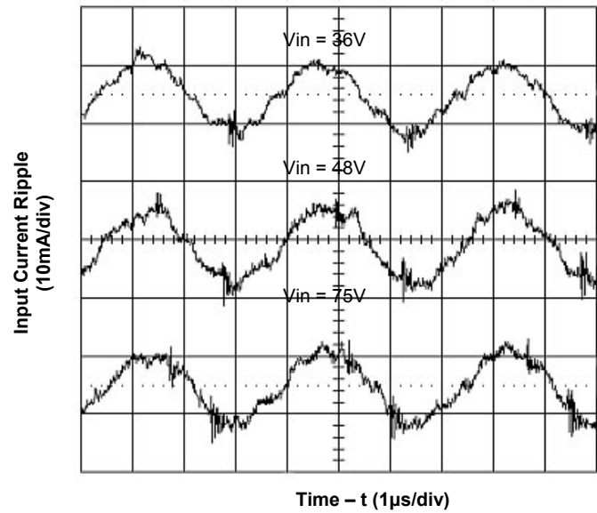
Figure 6. Input Reflected Ripple Current at 60A Load
