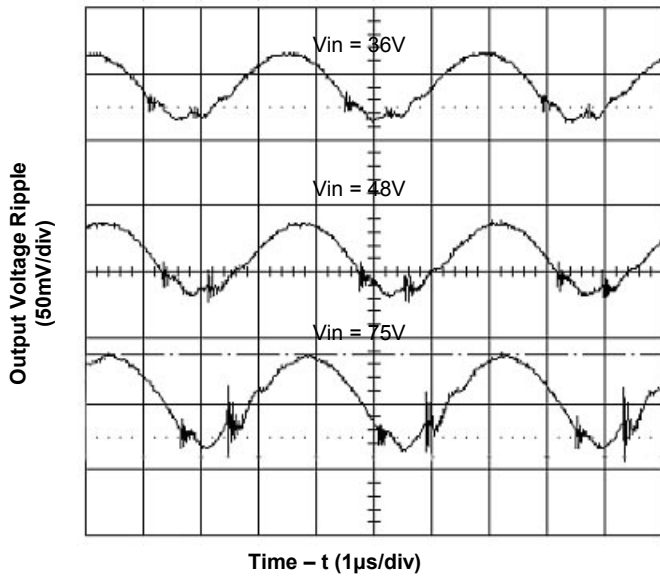
Figure 5. Output Ripple Voltage at 60A Load
