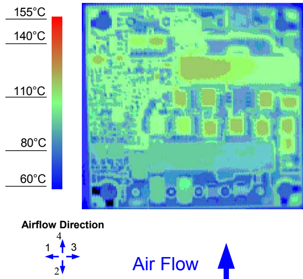
Figure 14. Thermal Image for Airflow Direction 4 (40.8A output, 55°C ambient, 200 LFM, Vin = 48V open frame unit using socket interface)
