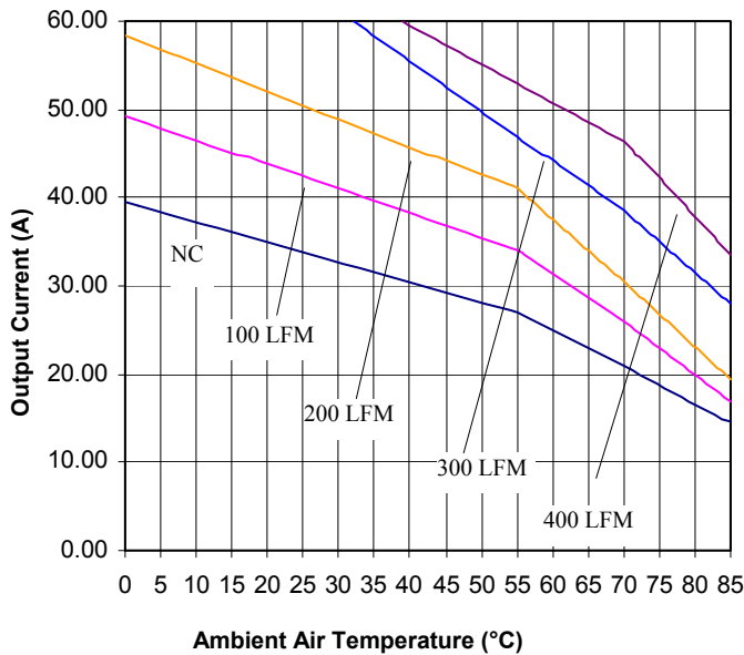
Figure 13. Current Derating Curve for Airflow Direction 4 (Ref. Fig. 14 for Airflow Direction; Vin = 48V open frame unit using socket interface)
