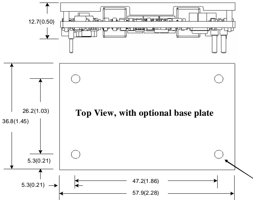
Figure 24. Converter with Optional Baseplate
