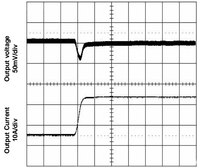
Time – t (500 \mu s/div) Figure 8. Transient Load Response
