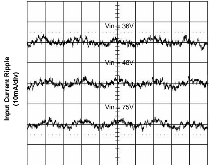
Time – t (2 \mu s/div) Figure 6. Input Reflected Ripple Current at 70A Load
