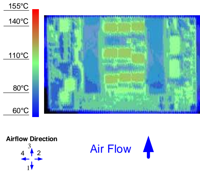
Figure 12. Thermal Image for Airflow Direction 3 (55A output, 55°C ambient, 200 LFM, V_{in} = 48V open frame unit using socket interface)
