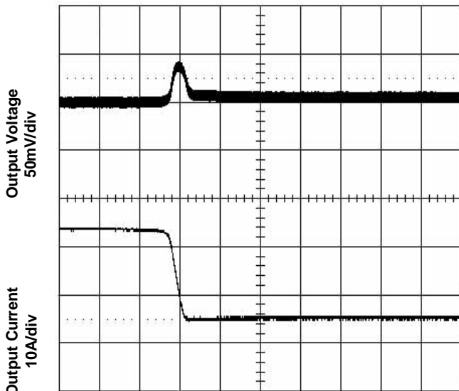
Time – t (500 \mu s/div) Figure 7. Transient Load Response
