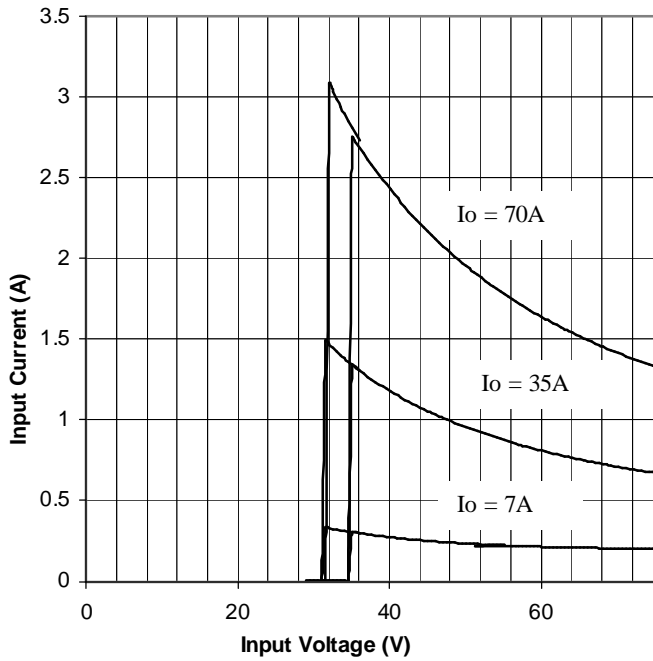
Figure 9. Input Characteristics
