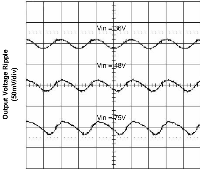
Time – t (2 \mu s/div) Figure 5. Output Ripple Voltage at 70A Load
