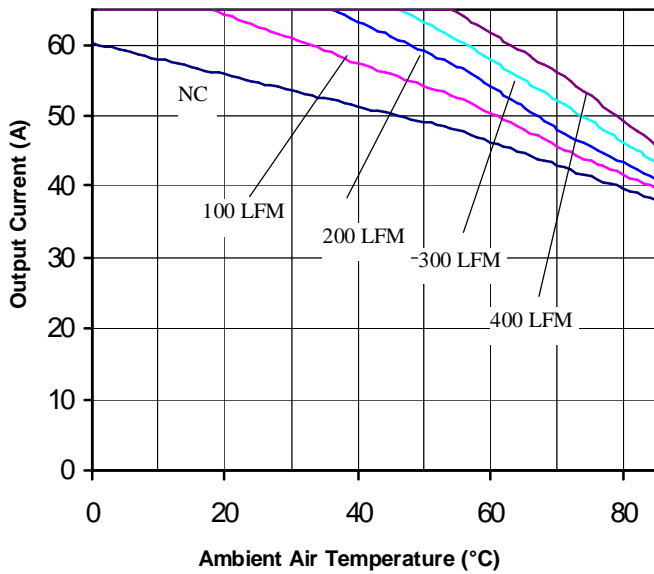
Figure 11. Current Derating Curve for Airflow Direction 3 (Ref. Fig. 12 for Airflow Direction; V_{in} = 48V open frame unit)
