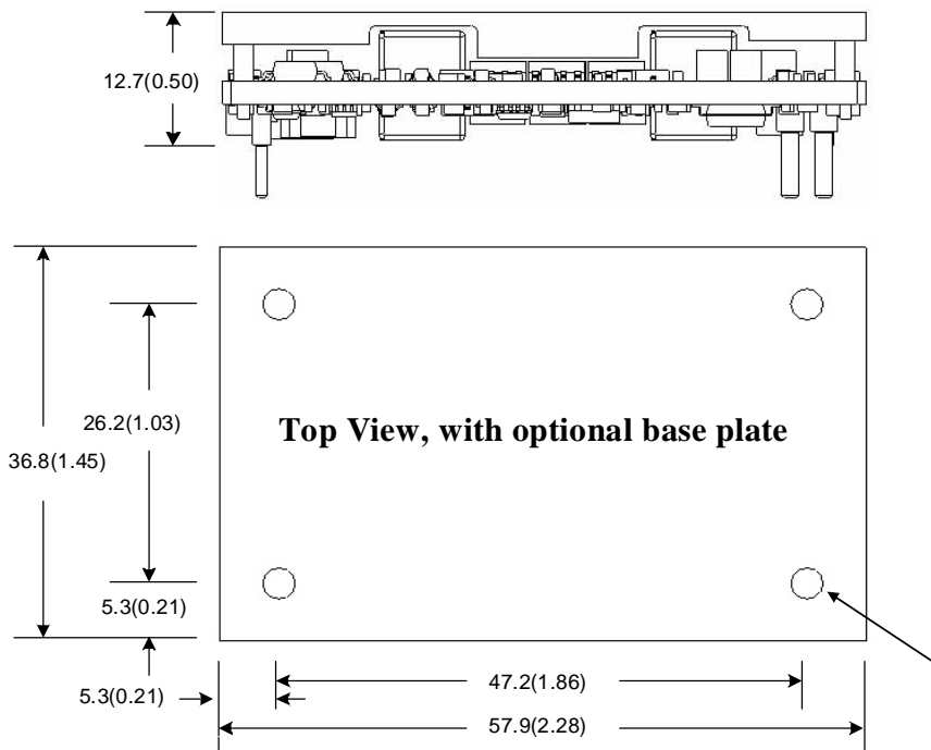
Figure 24. Converter with a baseplate
