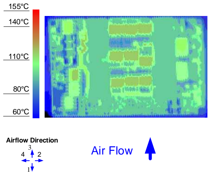
Figure 12. Thermal Image for Airflow Direction 3 (50A output, 55°C ambient, 200 LFM, V_{in} = 48V open frame unit using socket interface)
