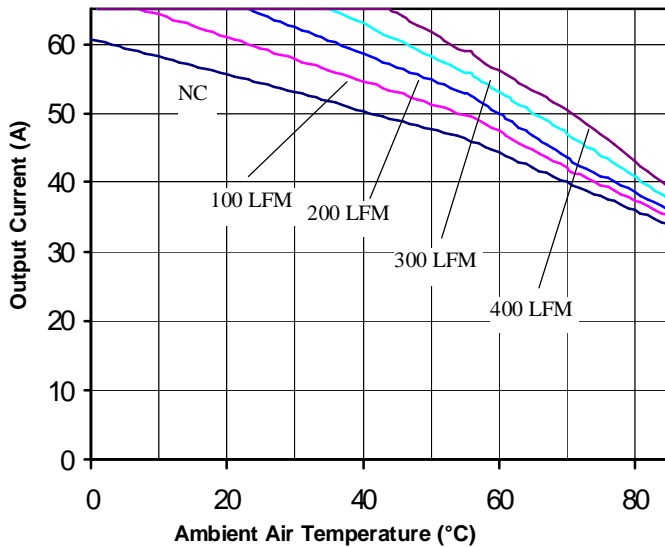
Figure 13. Current Derating Curve for Airflow Direction 2 (Ref. Fig. 14 for Airflow Direction; Vin = 48V open frame unit)
