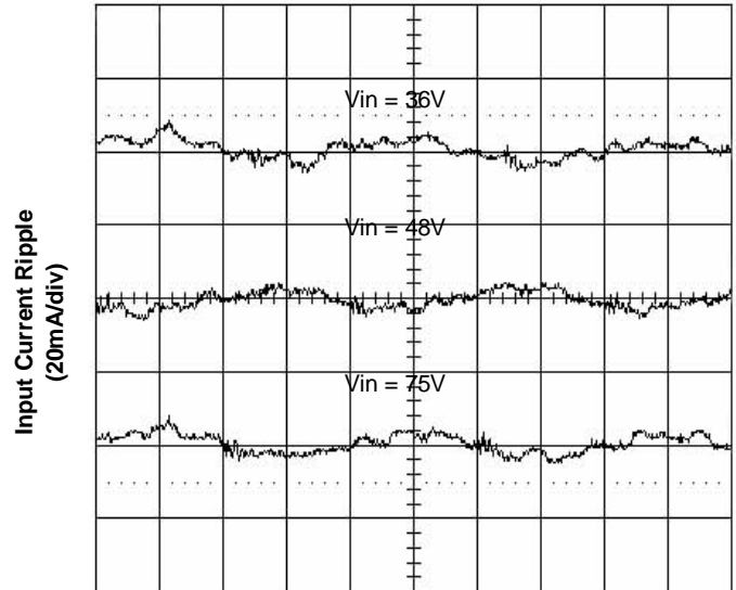
Time - t (1µs/div) Figure 6. Input Reflected Ripple Current at 65A Load
