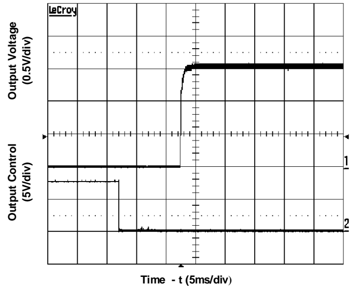
Figure 4. Start-Up from Enable Control
