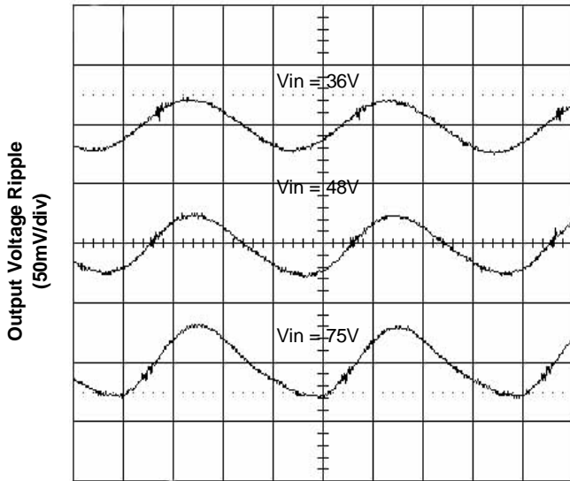
Time - t (1µs/div) Figure 5. Output Ripple Voltage at 65A Load
