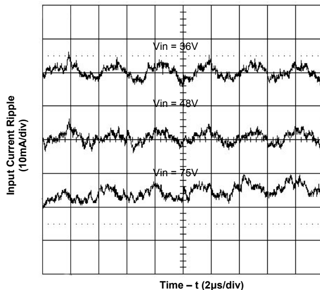
Figure 6. Input Reflected Ripple Current at 25A Load
