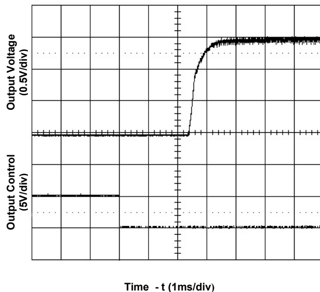
Figure 4. Start-Up from Enable Control
