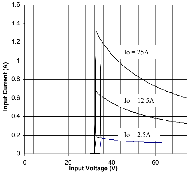
Figure 9. Input Characteristics
