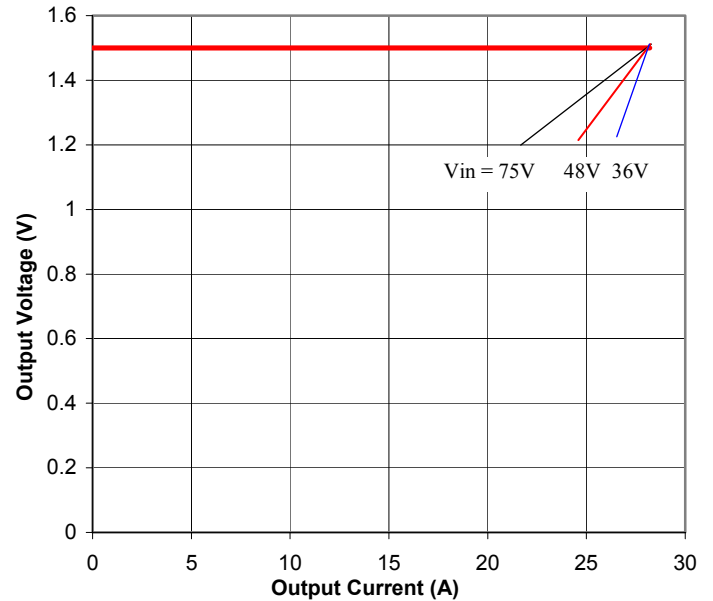
Figure 10. Output Characteristics
