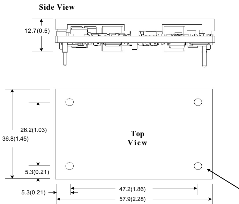
Figure 25. Converter with Optional Baseplate
