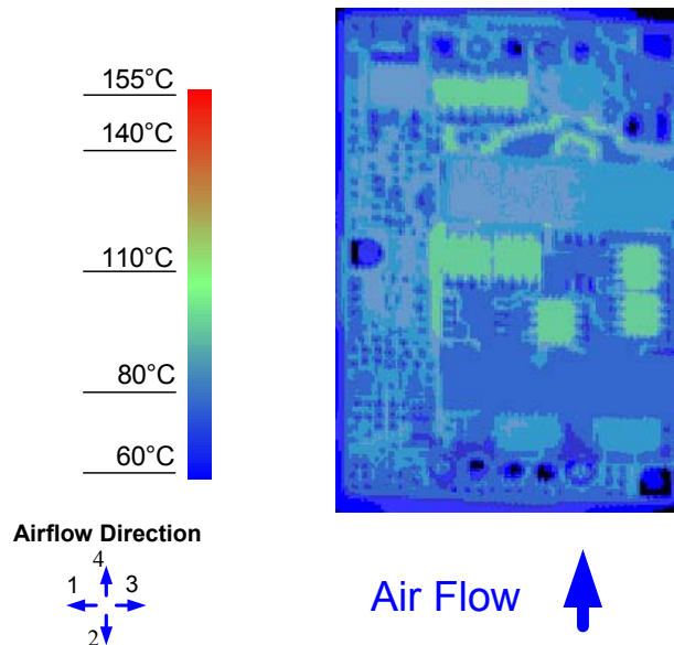
Figure 14. Thermal Image for Airflow Direction 4 (25A output, 55°C ambient, 200 LFM, Vin = 48V open frame unit using socket interface)
