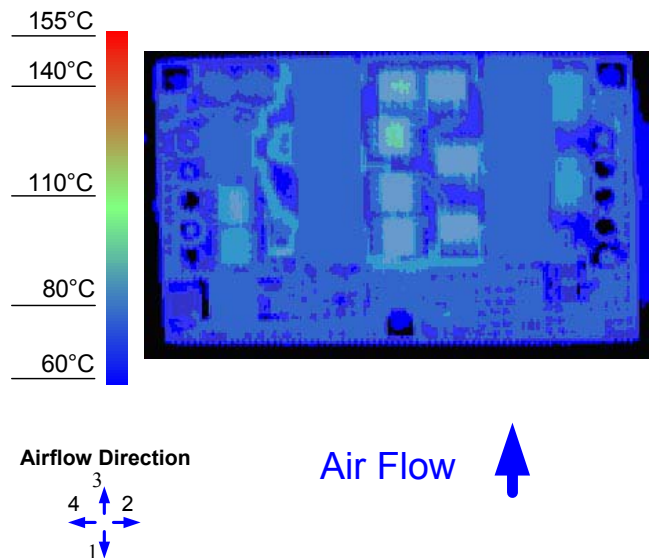
Figure 12. Thermal Image for Airflow Direction 3 (25A output, 55°C ambient, 200 LFM, Vin = 48V open frame unit using socket interface)
