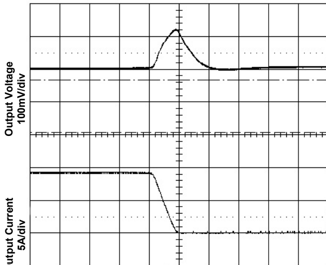
Time - t (100µs/div) Figure 7. Transient Load Response
