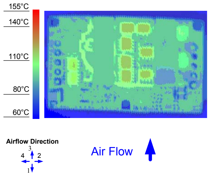
Figure 12. Thermal Image for Airflow Direction 3 (31.7A output, 55°C ambient, 200 LFM, V_{in} = 48V open frame unit using socket interface)
