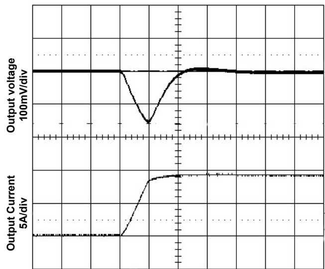
Time - t (100µs/div) Figure 8. Transient Load Response
