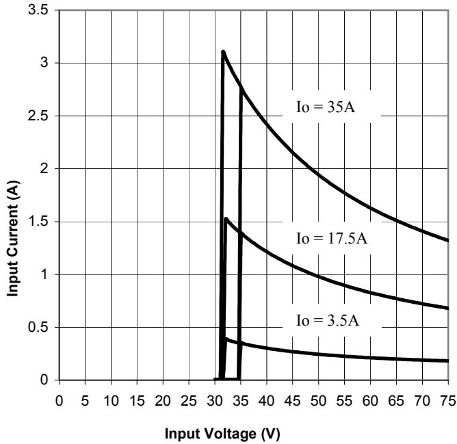
Figure 9. Input Characteristics
