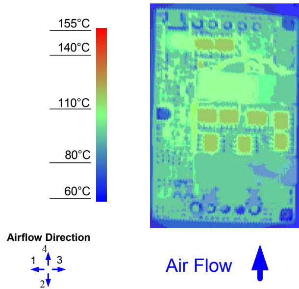
Figure 14. Thermal Image for Airflow Direction 4 (28A output, 55°C ambient, 200 LFM, Vin = 48V open frame unit using solder interface)
