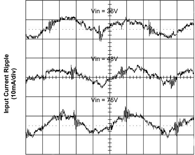
Time - t (1µs/div) Figure 6. Input Reflected Ripple Current at 35A Load
