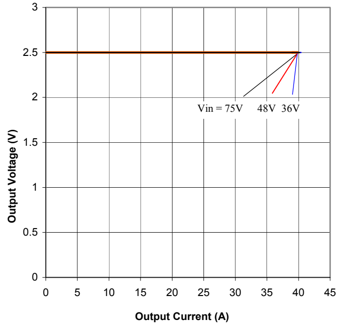
Figure 10. Output Characteristics
