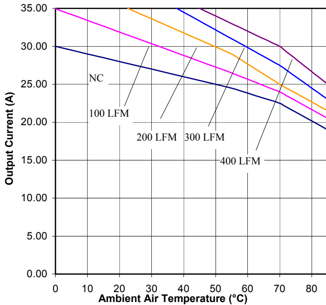
Figure 13. Current Derating Curve for Airflow Direction 4 (Ref. Fig. 14 for Airflow Direction; Vin = 48V open frame unit using socket interface )
