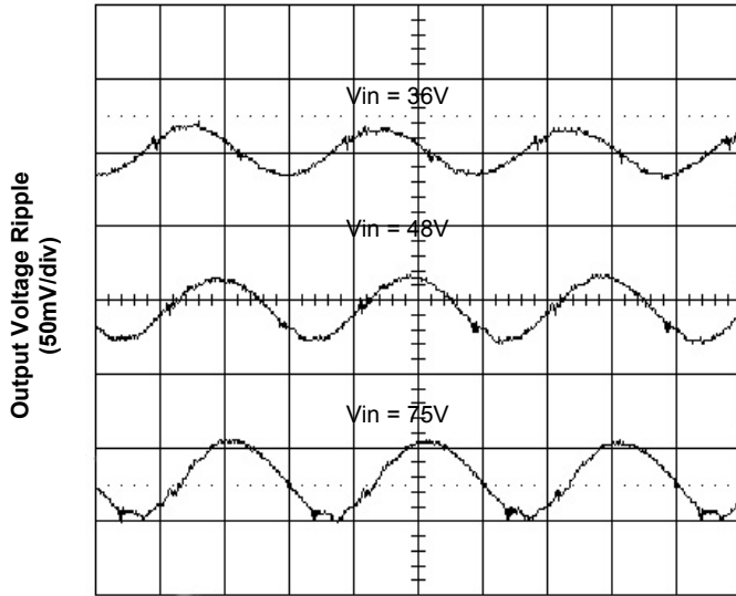
Time - t (1µs/div) Figure 5. Output Ripple Voltage at 35A Load
