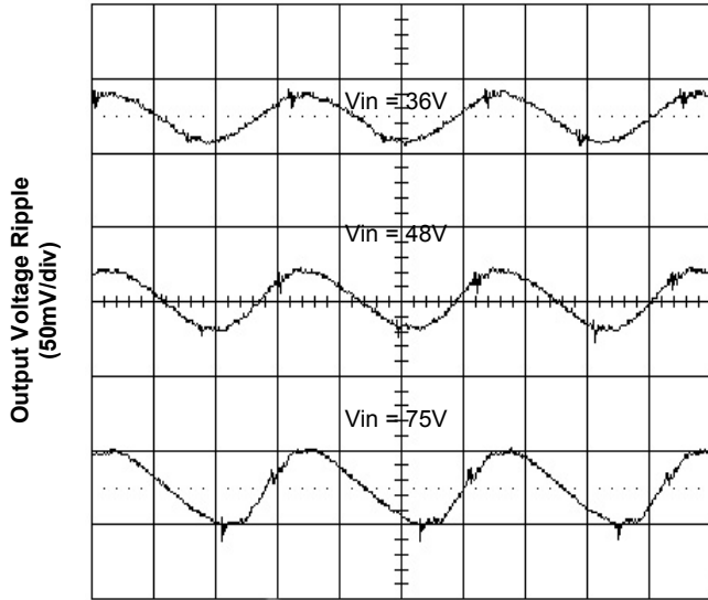
Time - t (1 \mu s/div) Figure 5. Output Ripple Voltage at 35A Load
