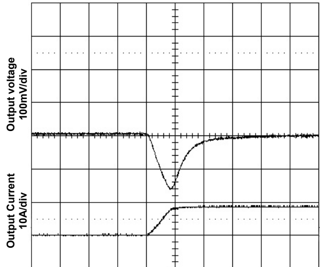
Time - t (100 \mu s/div) Figure 8. Transient Load Response
