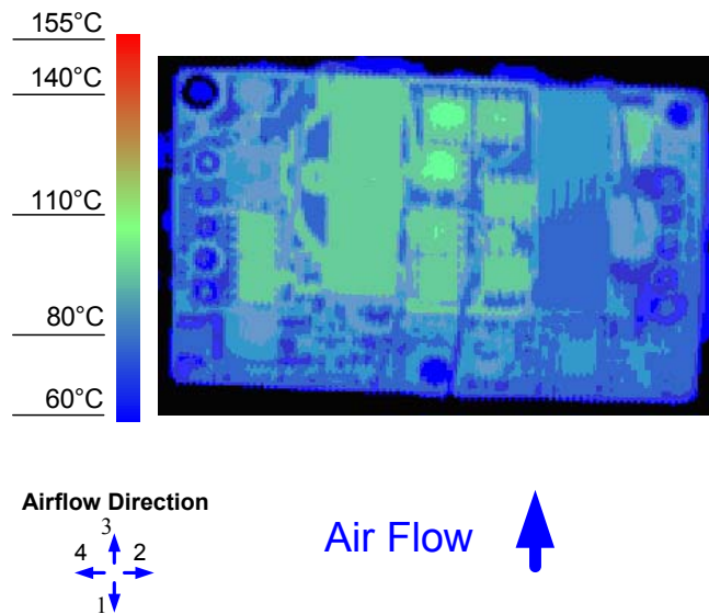
Figure 12. Thermal Image for Airflow Direction 3 (28A output, 55°C ambient, 200 LFM, V_{in} = 48V open frame unit using socket interface)
