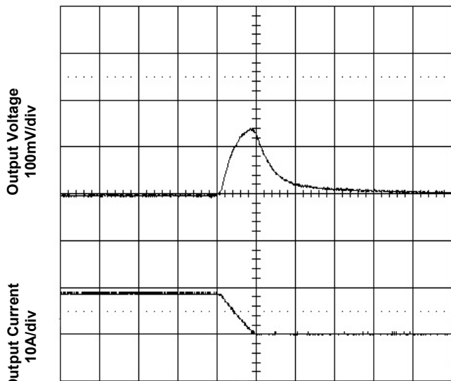
Time - t (100 \mu s/div) Figure 7. Transient Load Response
