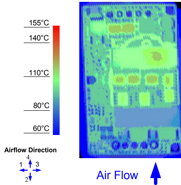
Figure 14. Thermal Image for Airflow Direction 4 (23A output, 55°C ambient, 200 LFM, Vin = 48V open frame unit using solder interface)
