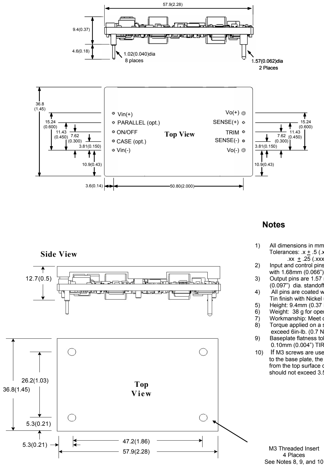
Figure 25. Converter with Optional Baseplate
