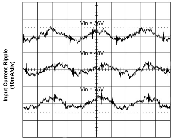
Time - t (1 \mu s/div) Figure 6. Input Reflected Ripple Current at 35A Load
