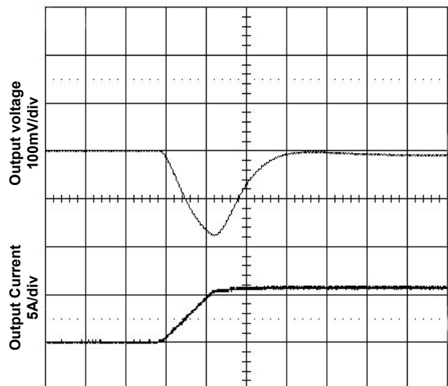
Time - t (50µs/div) Figure 8. Transient Load Response
