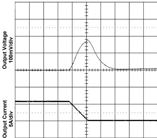
Time - t (50µs/div) Figure 7. Transient Load Response
