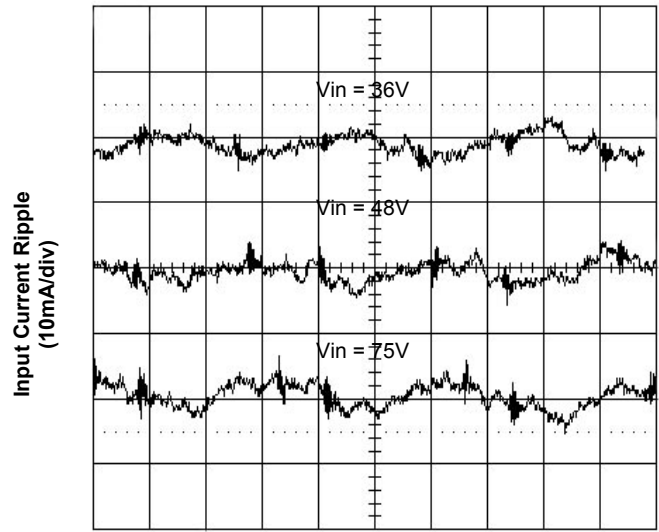
Time - t (1µs/div) Figure 6. Input Reflected Ripple Current at 25A Load
