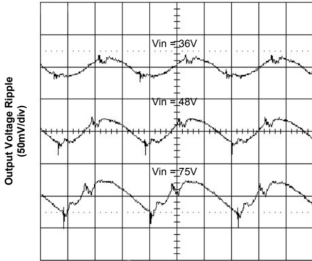
Time - t (1µs/div) Figure 5. Output Ripple Voltage at 25A Load
