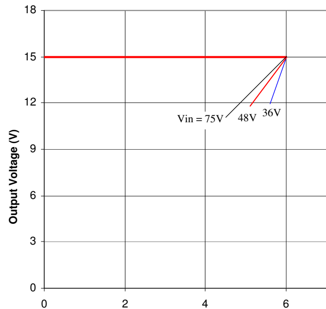
Figure 10. Output Characteristics
