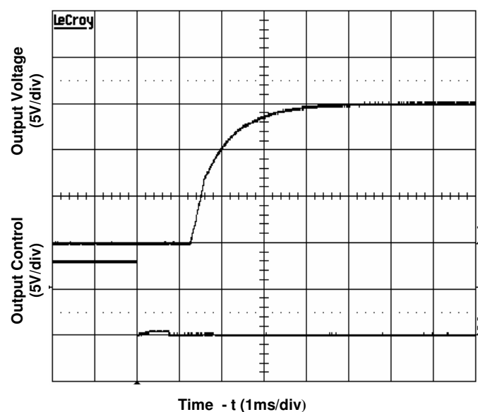
Figure 4. Start-Up from Enable Control Input voltage 48V, Output current 0A
