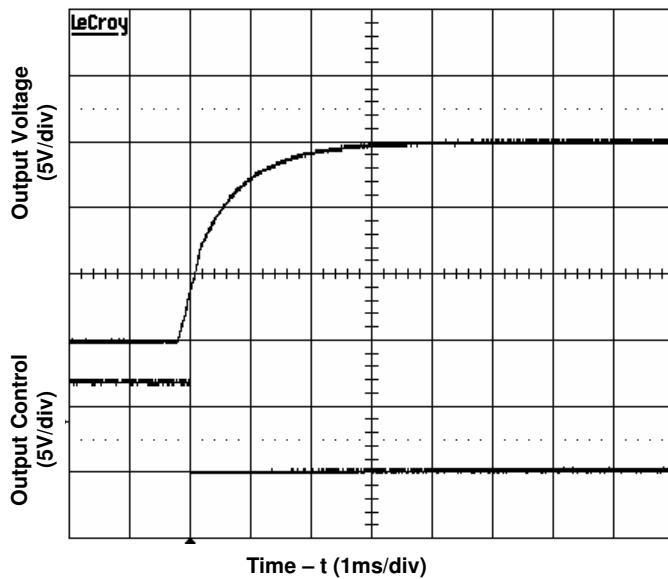
Figure 3. Start-Up from Enable Control Input voltage 48V, Output current 5A
