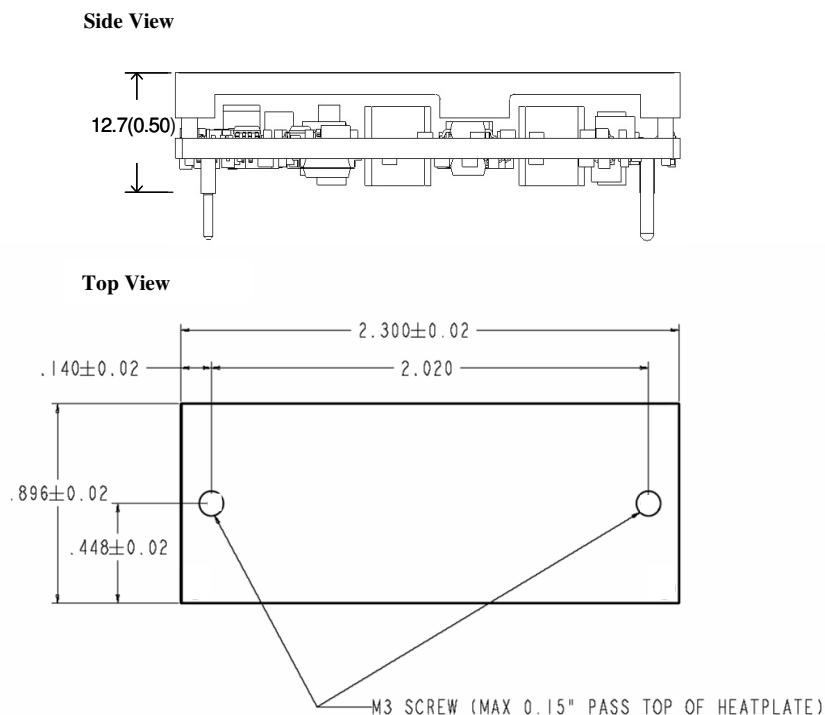
Figure 20. Converter with optional baseplate
