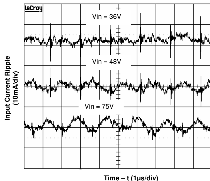
Figure 6. Input Reflected Ripple Current at 5A Load
