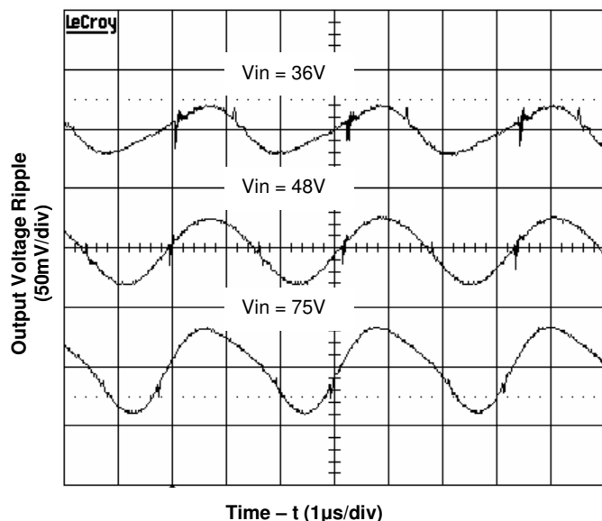
Figure 5. Output Ripple Voltage at 5A Load
