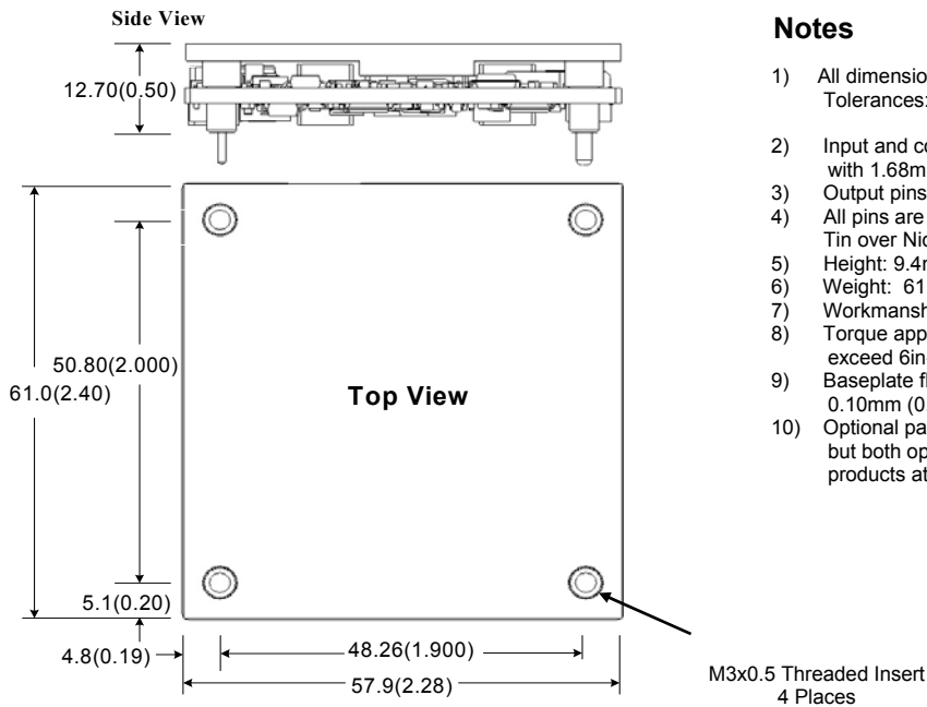
Figure 25. Converter with Optional Baseplate
