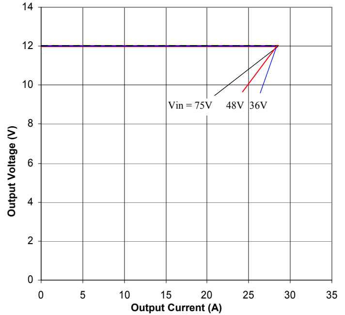
Figure 10. Output Characteristics
