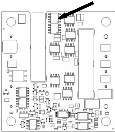
Figure 23. Temperature Monitoring Location
