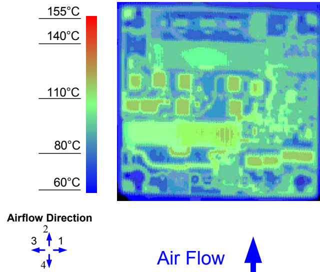
Figure 14. Thermal Image for Airflow Direction 2 (16A output, 55°C ambient, 200 LFM, Vin = 48V open frame unit using socket interface)
