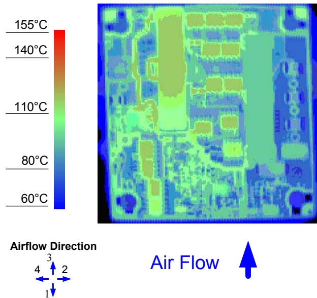
Figure 12. Thermal Image for Airflow Direction 3 (17.5A output, 55°C ambient, 200 LFM, V_{in} = 48V open frame unit using socket interface)
