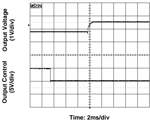
Figure 5. Start-Up with Prebias Input voltage 5V, Output current 0A, Output voltage 2.5V, Prebias 1.8V
