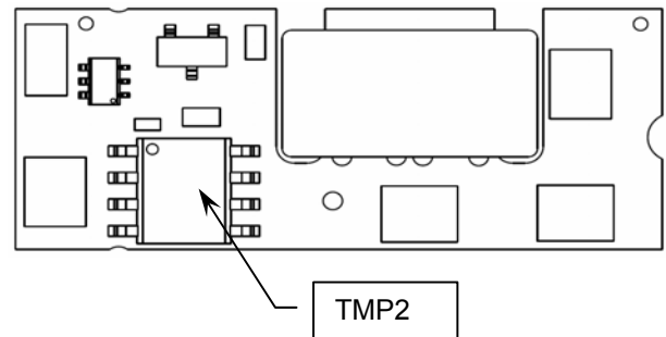
Figure 17. NBS Top View — Temperature Monitoring Point TMP2 for Derating Operation
