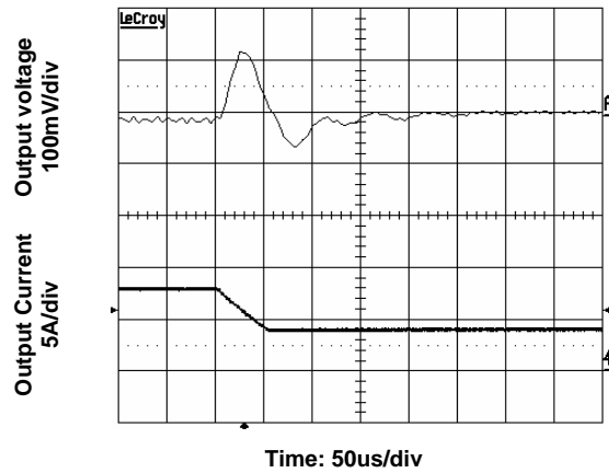
Figure 9. Transient Load Response. Output current 4A (50% full load), Input voltage 5V, Slew rate 0.2A/ \mu s.
