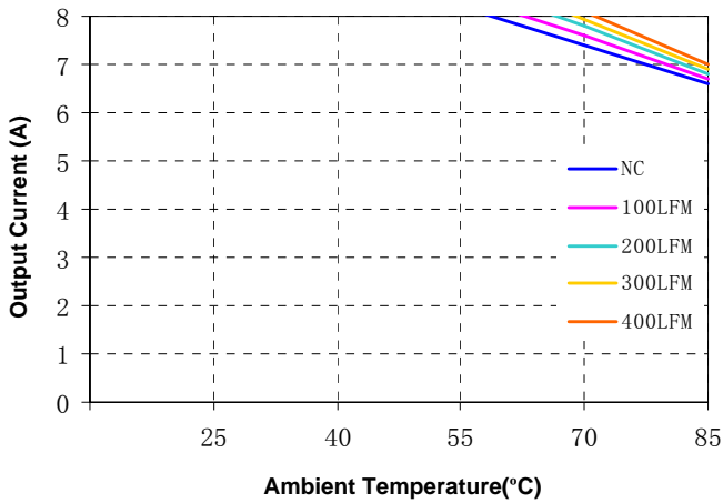
Figure 12(a). Current Derating Curve for 1.0V Output ( V_{in} = 5V open frame)
