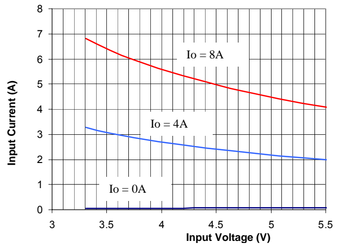
Figure 2. Input Characteristic (2.5V output)
