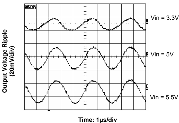
Figure 7. Output Ripple Voltage at 2.5V, 8A Output
