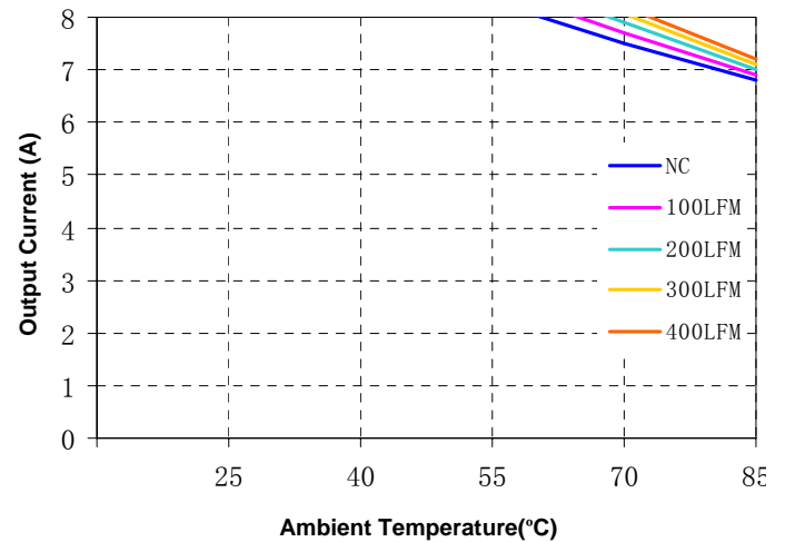
Figure 12(f). Current Derating Curve for 3.3V Output ( V_{in} = 5V open frame)
