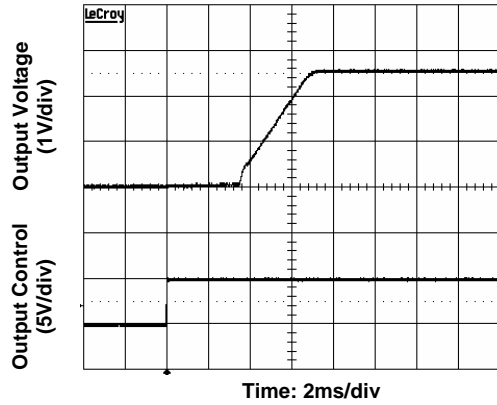
Figure 4. Start-Up from Application of Input Voltage Input voltage 5V, Output current 8A
