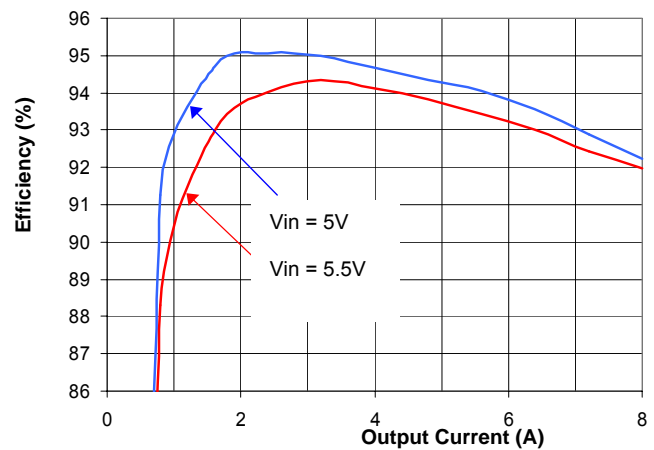
Figure 1(d). Efficiency vs. Load Current (25°C, 3.3V output)
