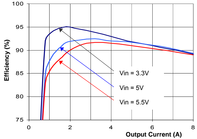
Figure 1(b). Efficiency vs. Load Current (25°C, 2.5V output)
