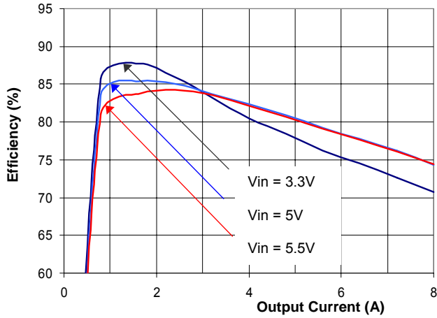
Figure 1(a). Efficiency vs. Load Current (25°C, 0.75V output)
