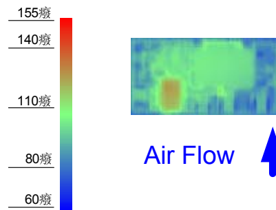
Figure 11. Thermal Image. V_{in} = 5V, 3.3V/8A output, 55°C ambient, 200 LFM
