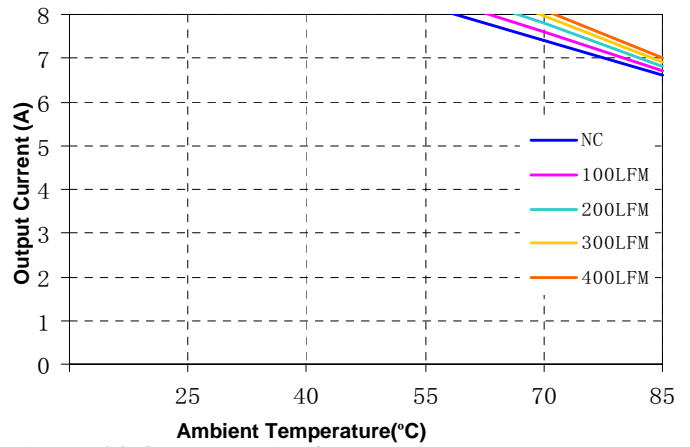
Figure 12(b). Current Derating Curve for 1.2V Output ( V_{in} = 5V open frame)
