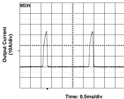
Figure 8. Short circuit current. Vin = 5V.
