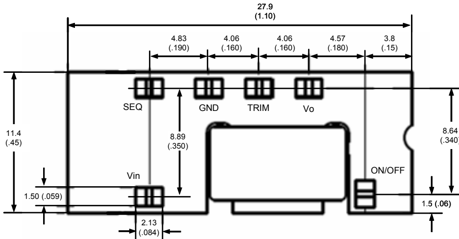
Bottom View
