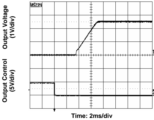
Figure 3. Start-Up from Enable Control Input voltage 5V, Output current 8A
