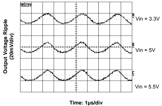
Figure 6. Output Ripple Voltage at 1V, 8 A Output
