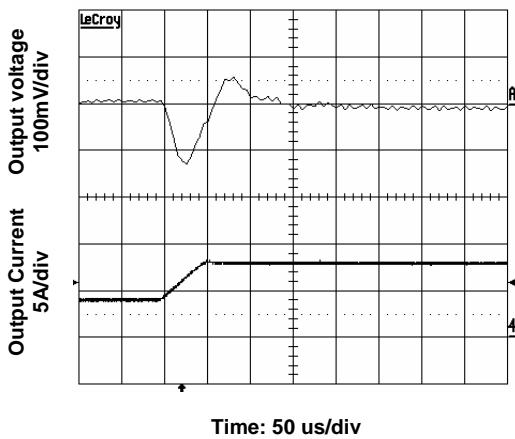
Figure 8. Transient Load Response. Output current 4A (50% full load), Input voltage 5V, Slew rate 0.2A/ \mu s.
