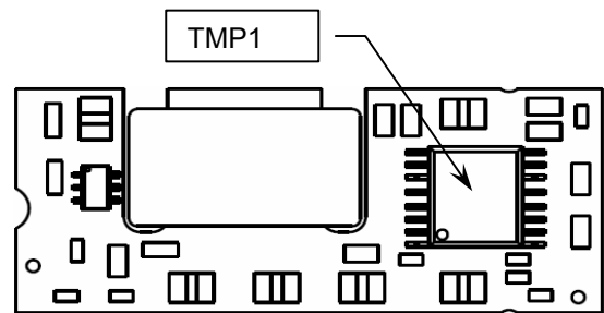
Figure 16. NBS Bottom View — Temperature Monitoring Point TMP1 for Thermal Shutdown
