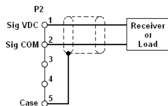
VOLTAGE OUTPUT
