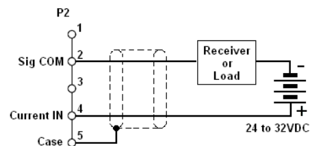
4.20mA OUTPUT USING AN EXTERNAL LOOP SUPPLY
