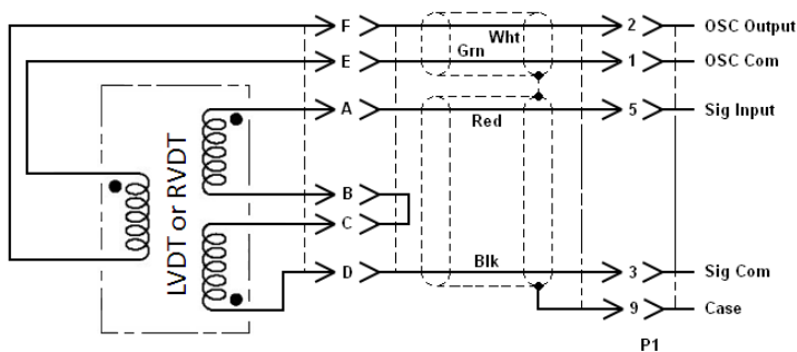
TRANSDUCER WITH CONNECTOR AND JUMPER CABLE
