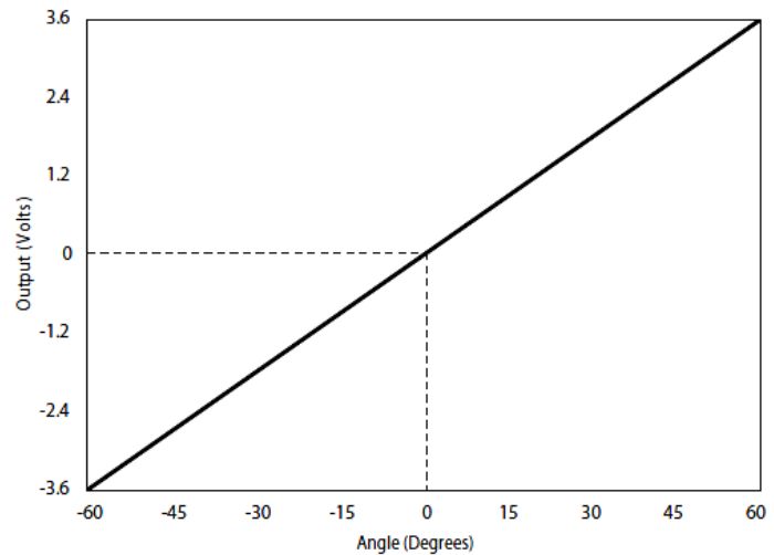
Analog Output
