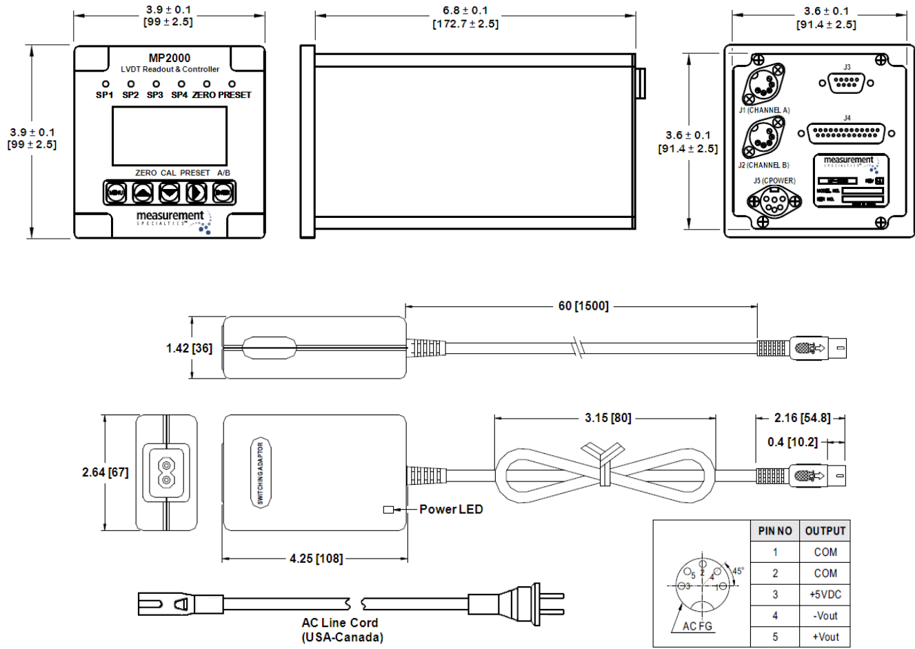
Dimensions are in inch [mm]
